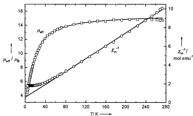
Figure 3. The effective magnetic moment ( \mu_{\text{eff}} ) and the inverse susceptibility \chi_{\text{m}}^{-1} data as a function of temperature for 2 . Open points represent observed results, and solid lines for \chi_{\text{m}}^{-1} and \mu_{\text{eff}} represent the fitting curves based on the Curie – Weiss law and on a simplified exchange fit as described in the text, respectively.
